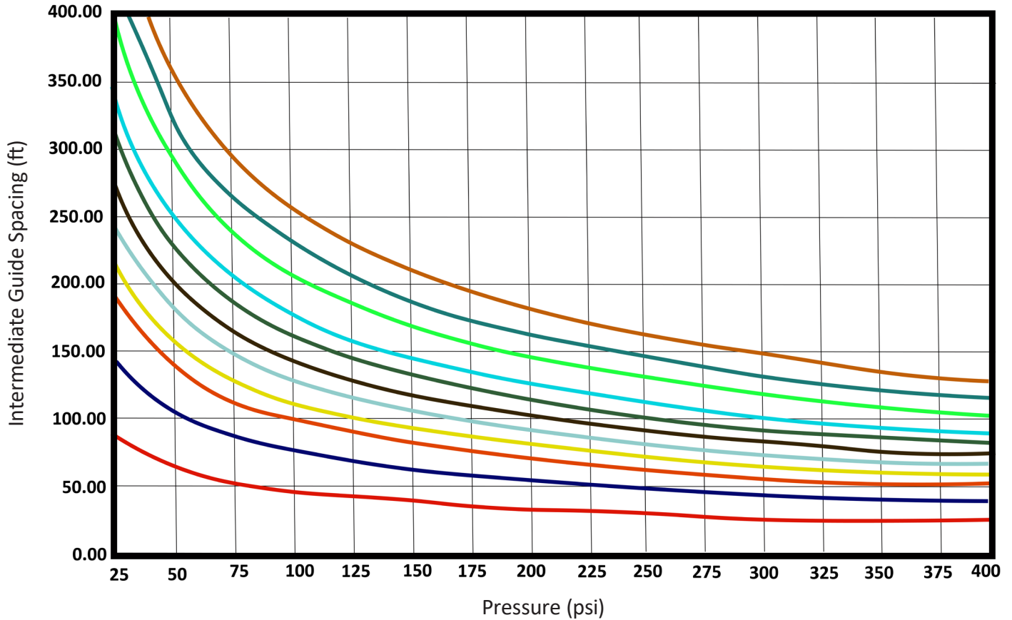
Recommended Maximum Spacing of Intermediate Pipe Guides for Applications Involving Axial Movement
